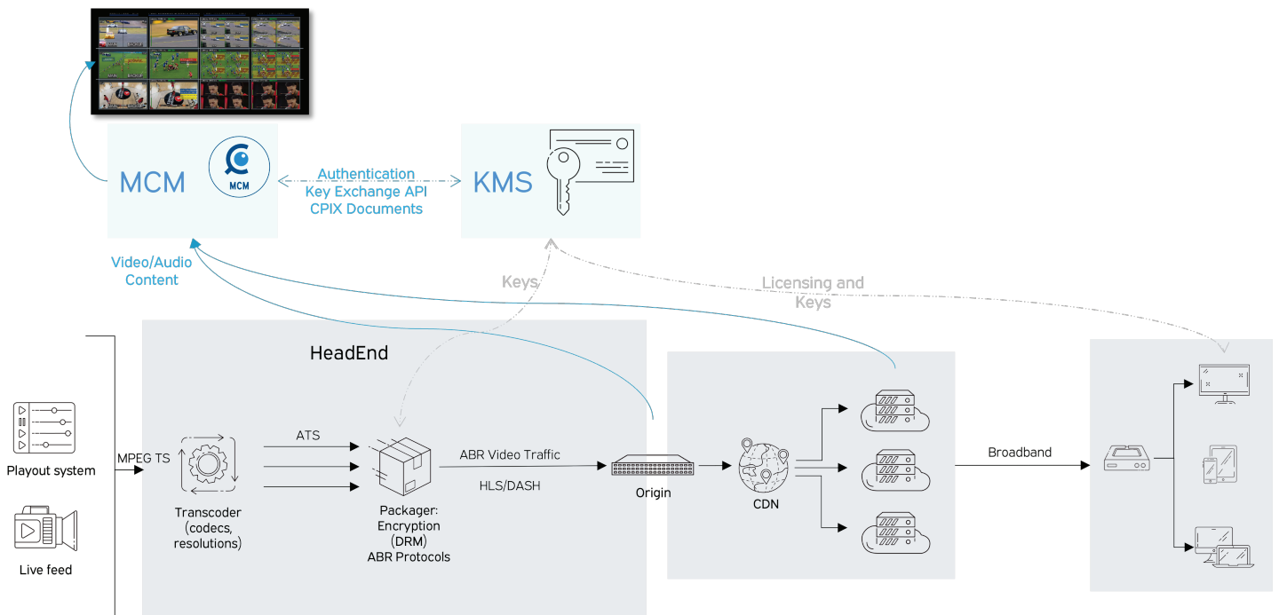
Figure 1 - KMS Integration (TAG MCM)
